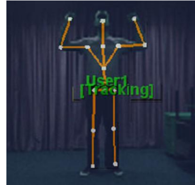
Figure 1. The psi-pose
